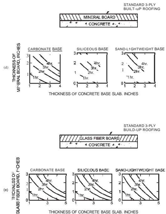
FIGURE 721.2.2.3(1) FIRE-RESISTANCE RATINGS FOR CONCRETE ROOF ASSEMBLIES
