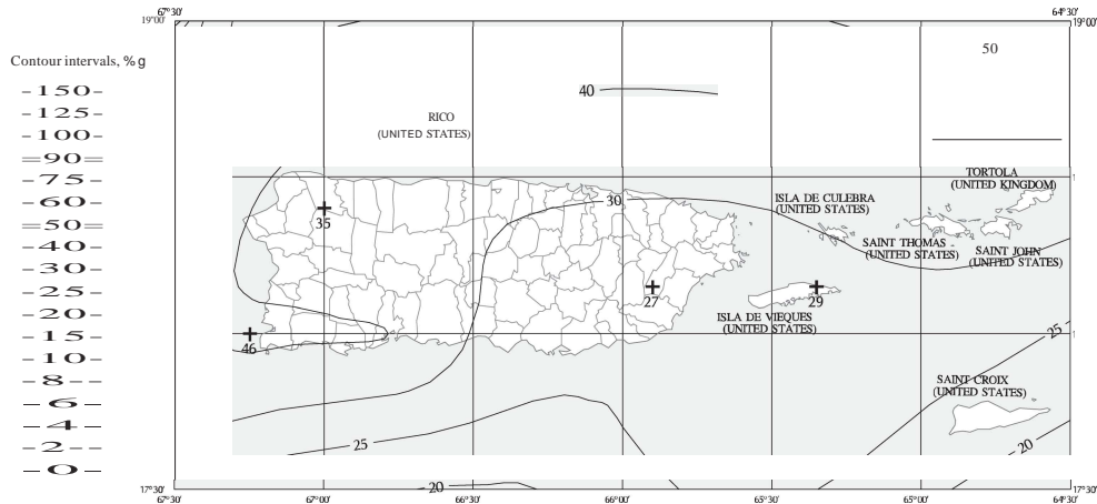
1.0 SEC SPECTRAL RESPONSE ACCELERATION (5% OF CRITICAL DAMPING)
