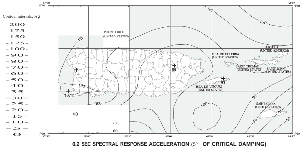
0.2 SEC SPECTRAL RESPONSE ACCELERATION (5% OF CRITICAL DAMPING)
